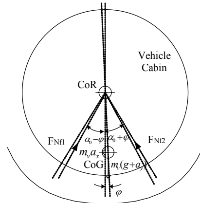
Fig. 6 Length Compensation Control Model
