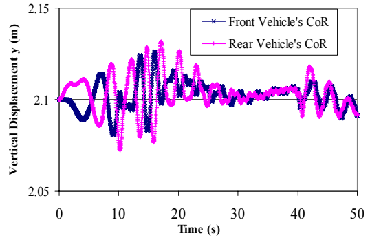
Fig. 9 Lateral and Vertical Displacements of Front and Rear Vehicle's CoR
