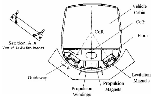
Fig. 1 Front View of Vehicle and Guideway
