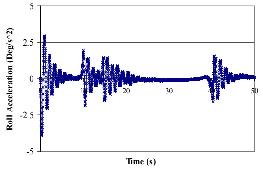
Fig. 12 Roll Acceleration
