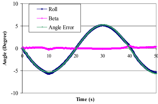
Fig. 11 Roll, Beta and Angle Error
