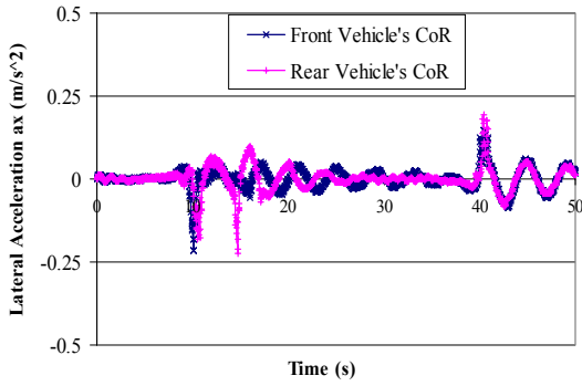
Fig. 10 Lateral and Vertical Accelerations of Front and Rear Vehicle's CoR
