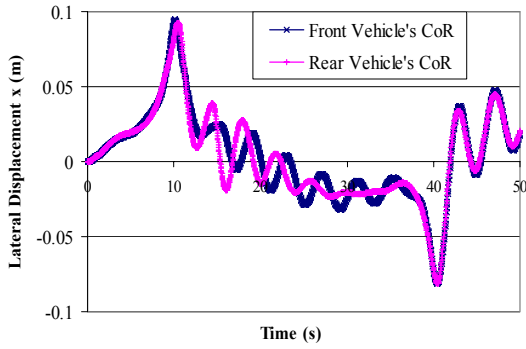
Fig. 9 Lateral and Vertical Displacements of Front and Rear Vehicle's CoR
