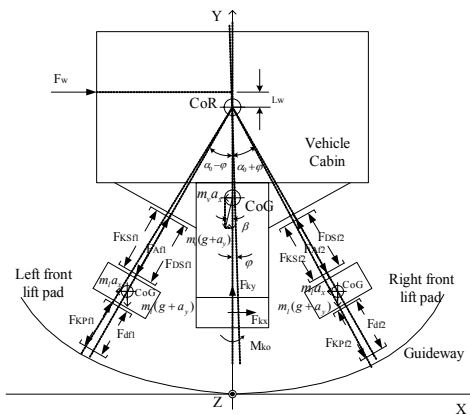
Fig. 3 Front View of 3D Vehicle Dynamic Model
