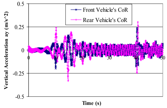
Fig. 10 Lateral and Vertical Accelerations of Front and Rear Vehicle's CoR
