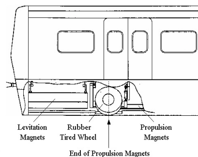
Fig. 2 Side View of Vehicle
