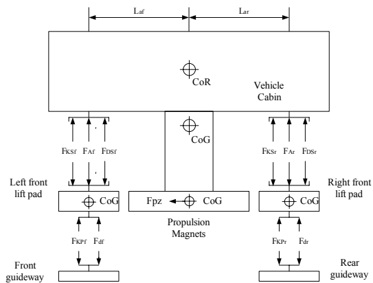
Fig. 4 Side View of Vehicle Force Model
