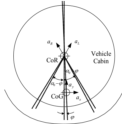
Fig. 5 Acceleration Feedback Model
