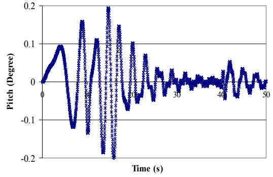
Fig. 14 Pitch Angle
