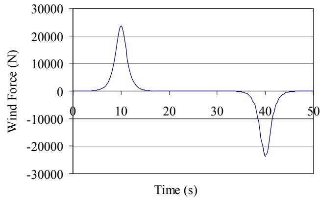
Fig. 8 Strong Wind Forces
