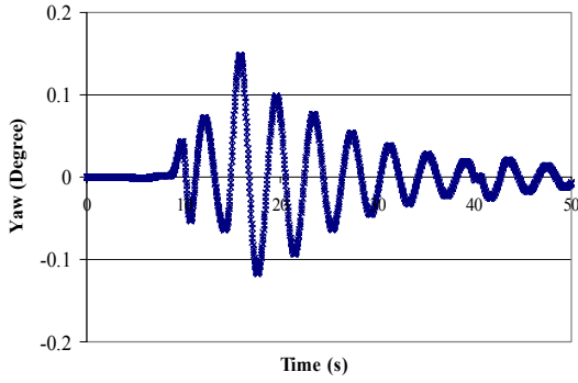
Fig. 13 Yaw Angle
